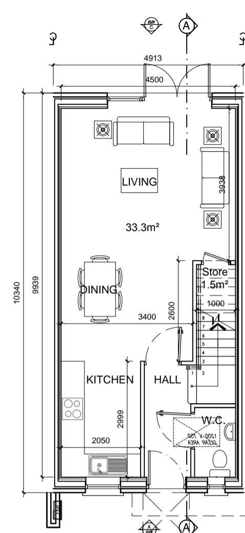
GROUND FLOOR PLAN Right Entry area 43.6m² / 469 ft² O/ALL AREA 86.6m² / 932 ft²
