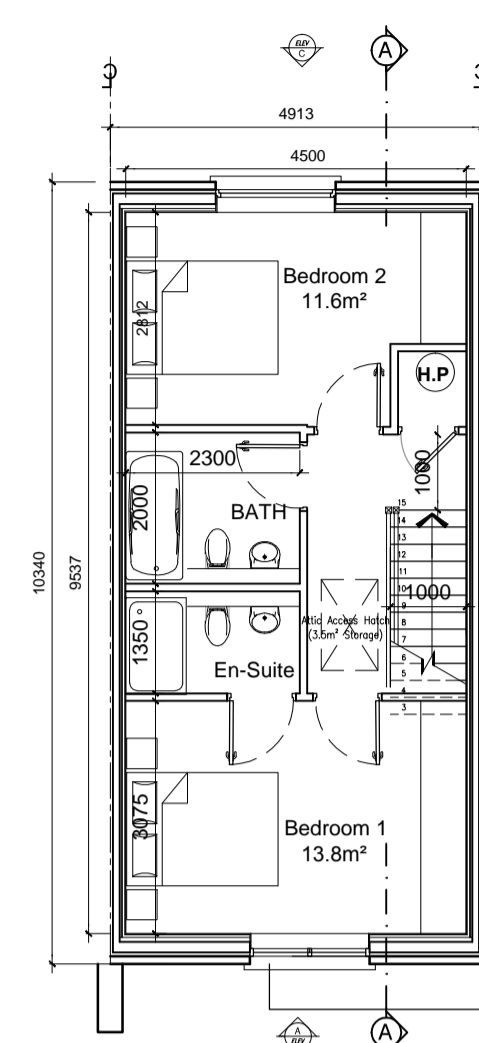
FIRST FLOOR PLAN Right Entry area 43m² / 463 ft²
