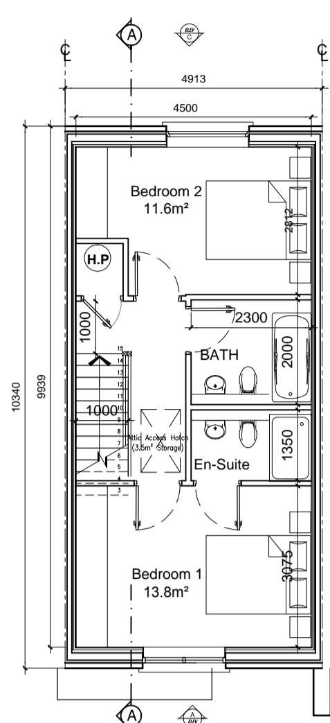
FIRST FLOOR PLAN Left Entry area 43m² / 463 ft²
