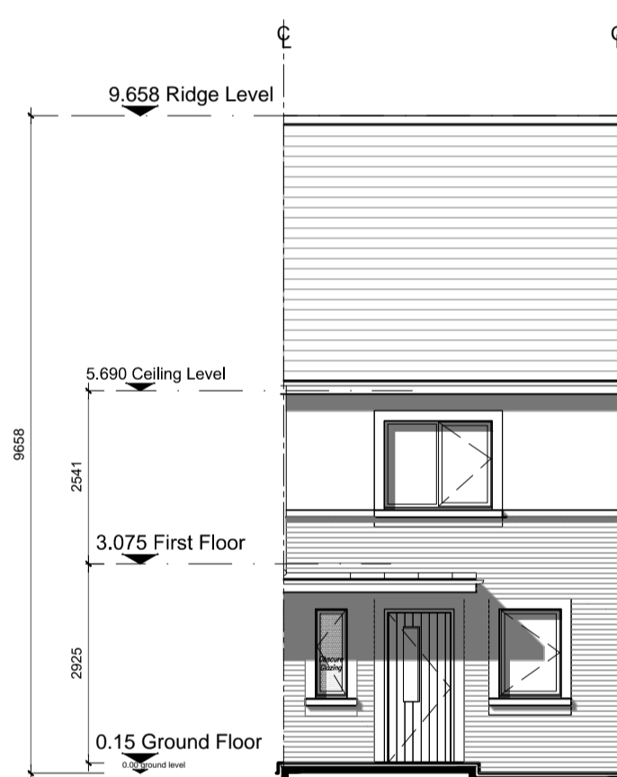
Front Elevation 'A' Left Entry
