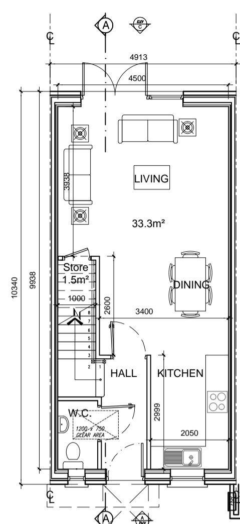
GROUND FLOOR PLAN Left Entry area 43.6m² / 469 ft² O/ALL AREA 86.6m² / 932 ft²
